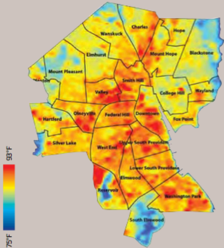
Daytime Surface Temperature August 3, 2006, 11:20am
